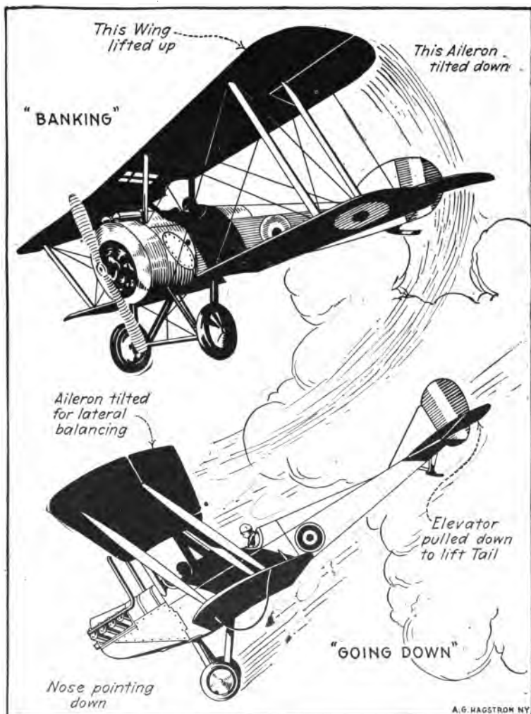
Fig. 97. Illustrations Showing How Control Elements are Moved to Regulate Airplane Flight.
