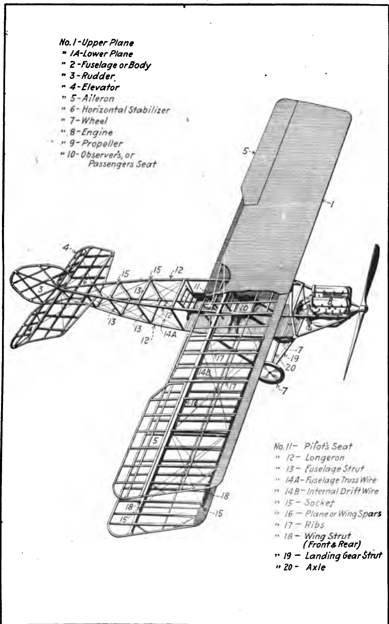
PLATE I.—Part Sectional View of Typical Airplane, Showing Important Parts.
