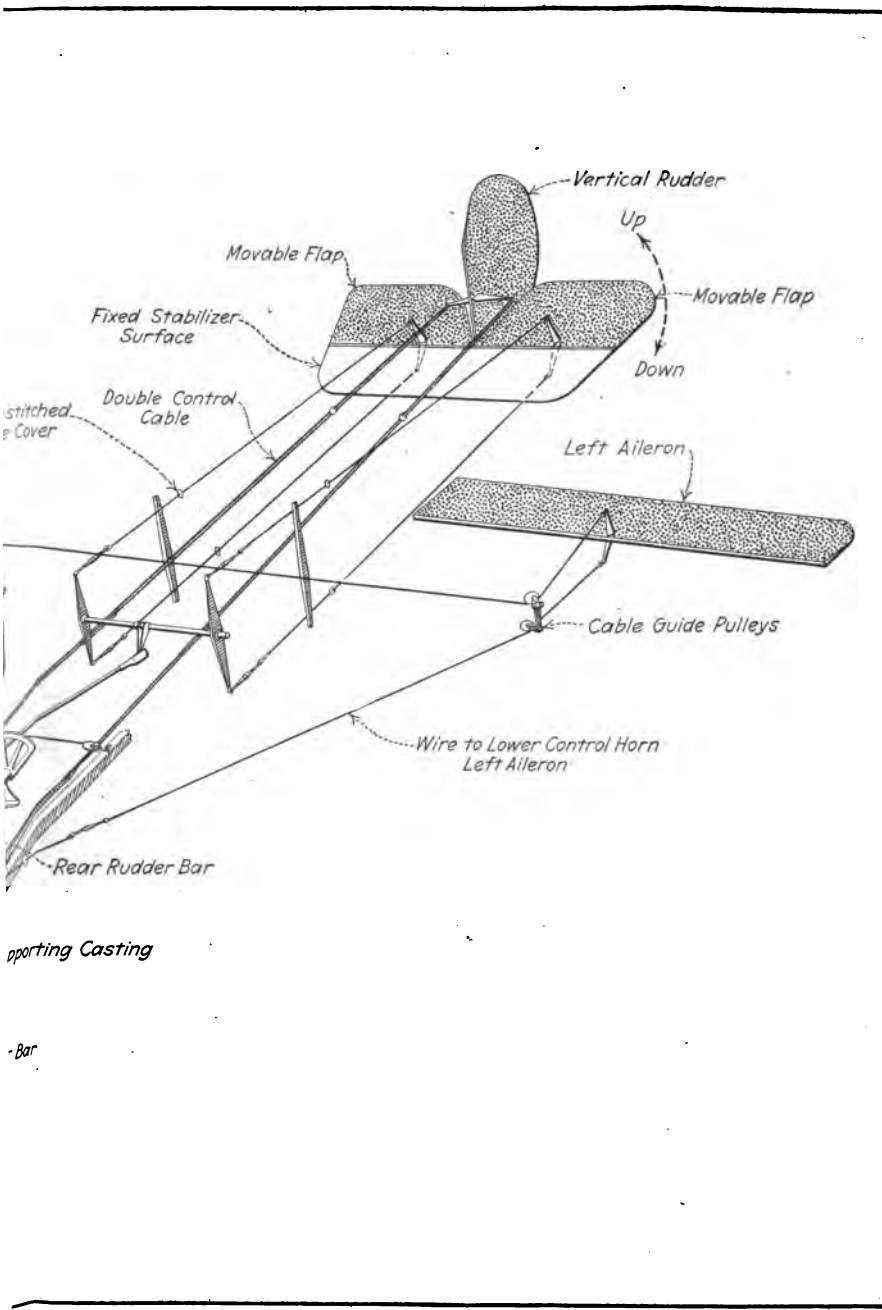
Showing all Cables and Control Members.
