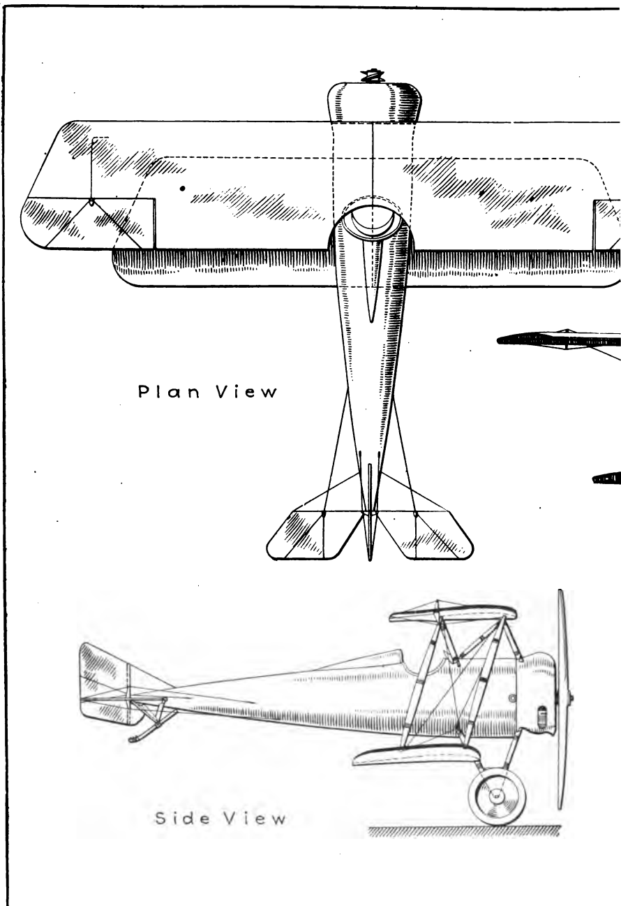
Fig. 114. Design Drawings of Berkman Speed Scout, a Single-Seat, High Speed
