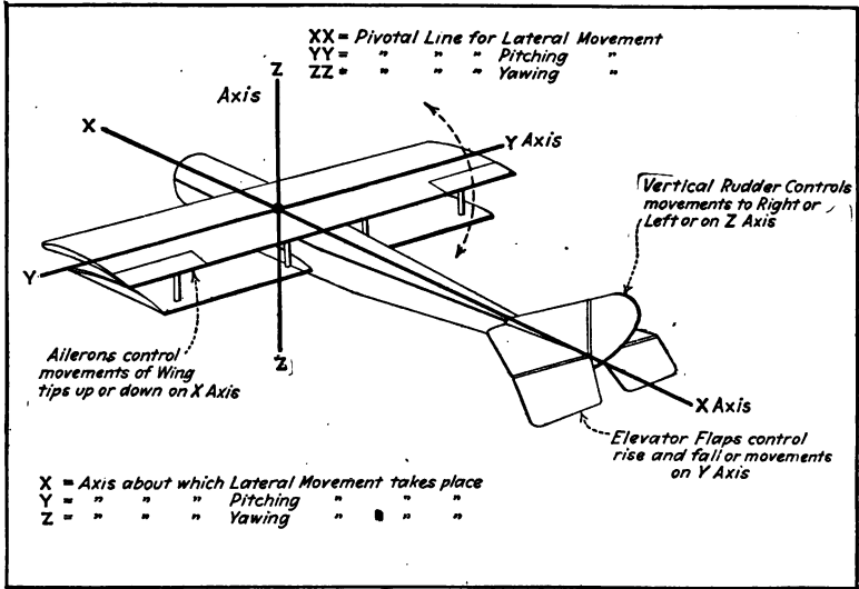
Fig. 84. A Diagrammatic Representation of the Three Axes about Which Movement of an Airplane in Flight May Take Place.
