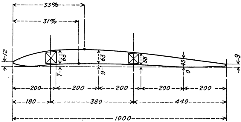
Wing Section of the Sopwith Triplane
