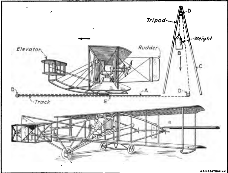
Fig. 50. Two Early Biplanes, That at the Top being the Historic Wright Machine Which Demonstrated the Possibilities of Mechanical Flight. The Lower One is an Early Curtiss Machine of Remarkably Dependable Characteristics.
