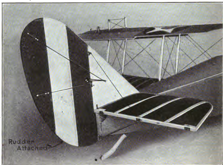
Fig. 109. Rear View of Fuselage with Vertical Rudder in Place.
