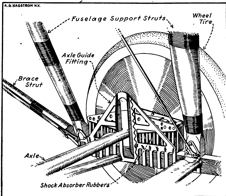
Fig. 59. Landing Gear Parts for Heavy Machine.
